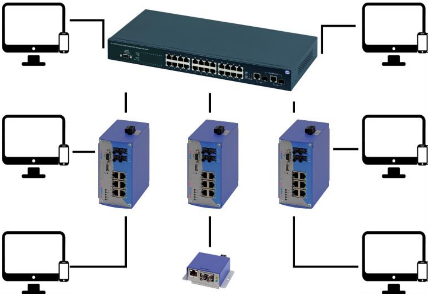
Figure 6: EL-100-2MA in a star-shaped network
