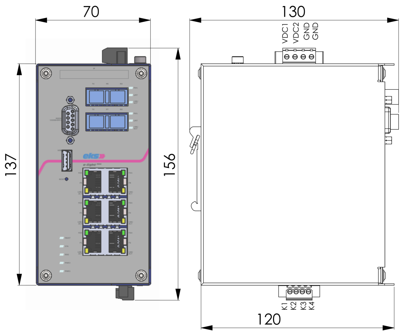
Figure 5: Dimensions of the EL-100-2MA switch
