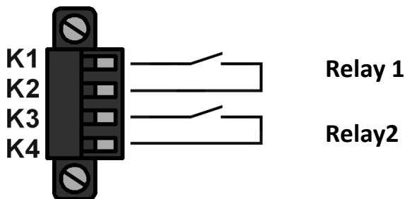
Figure 3: Relay terminal clamp
