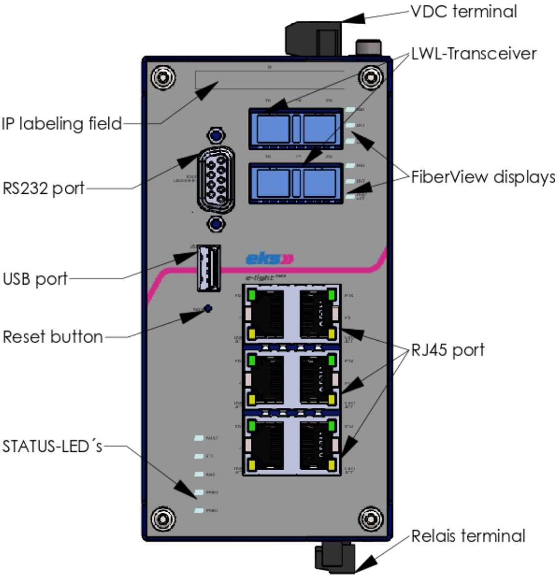
Figure 1: Front view of the EL-100-2MA switch with 2 LWL transceivers
