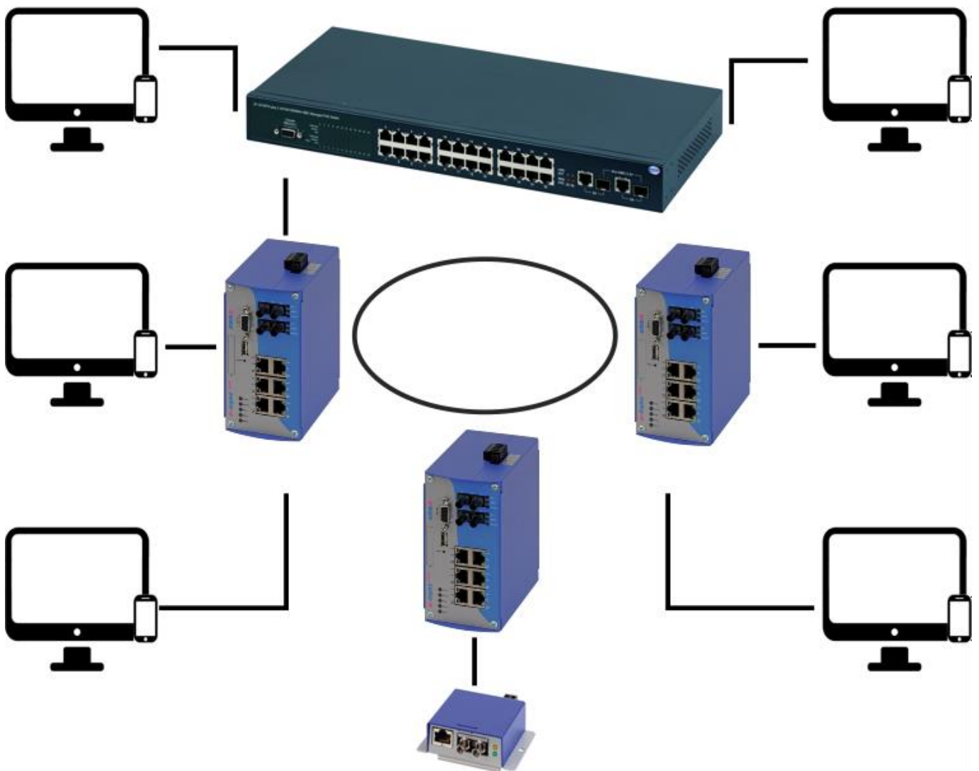
Figure 8: EL-100-2MA in a ring-shaped network
