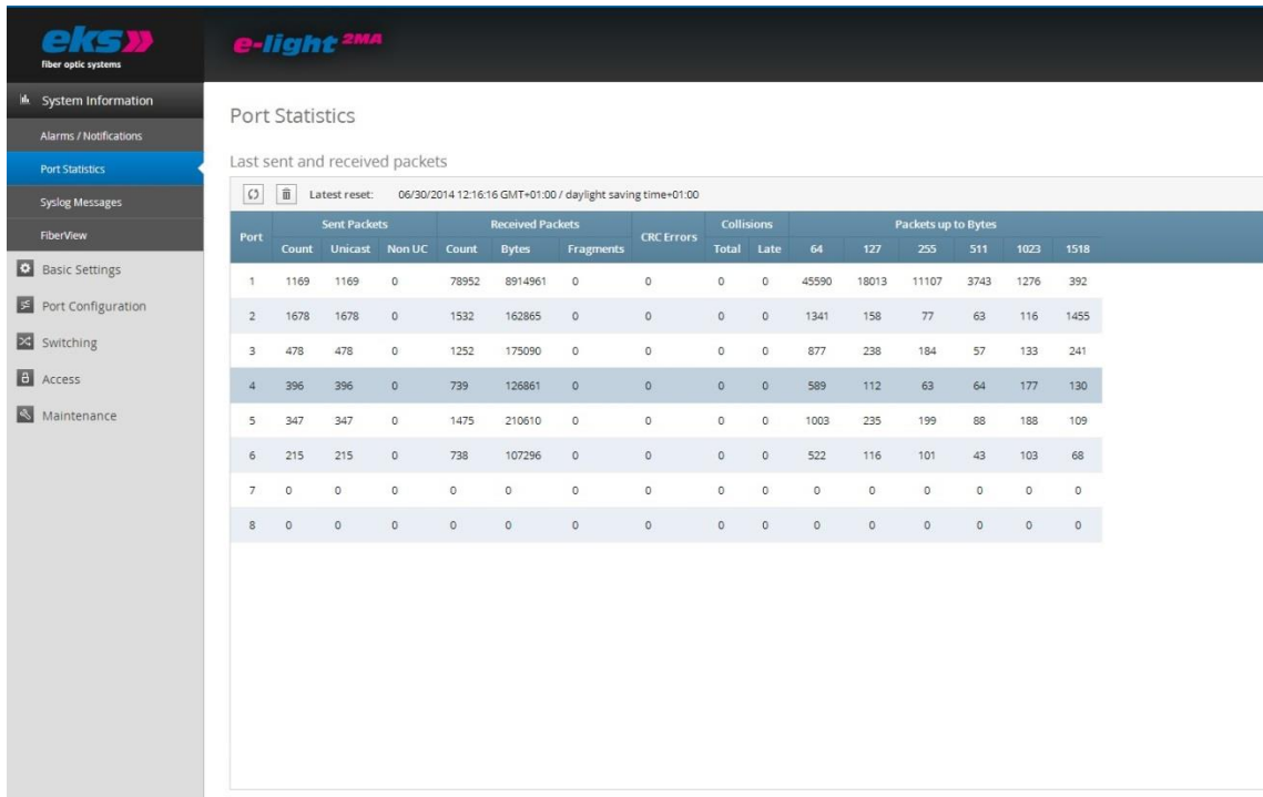
Figure 13: Port statistics
