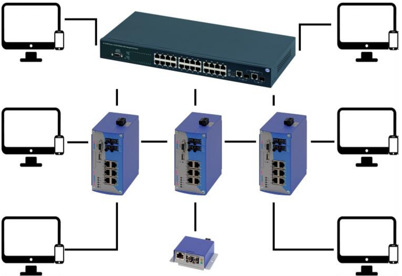
Figure 7: EL-100-2MA in a meshed network
